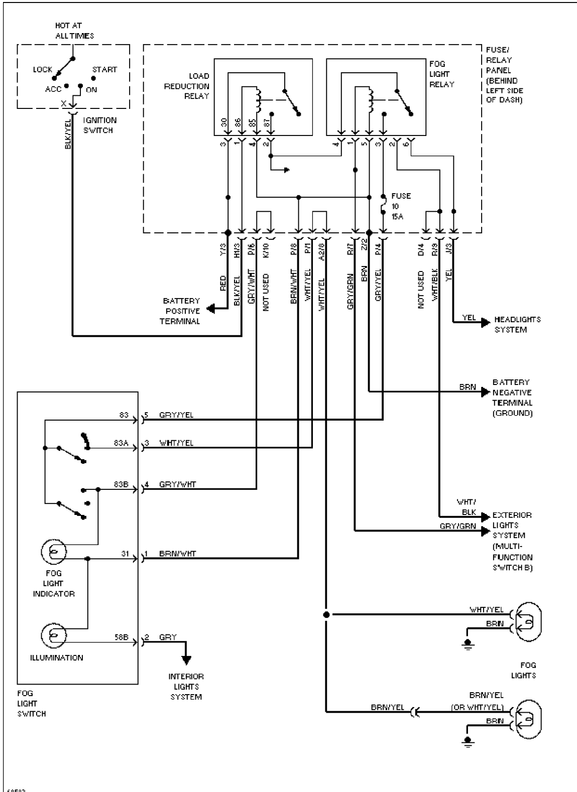
Fog Lamp Circuit
