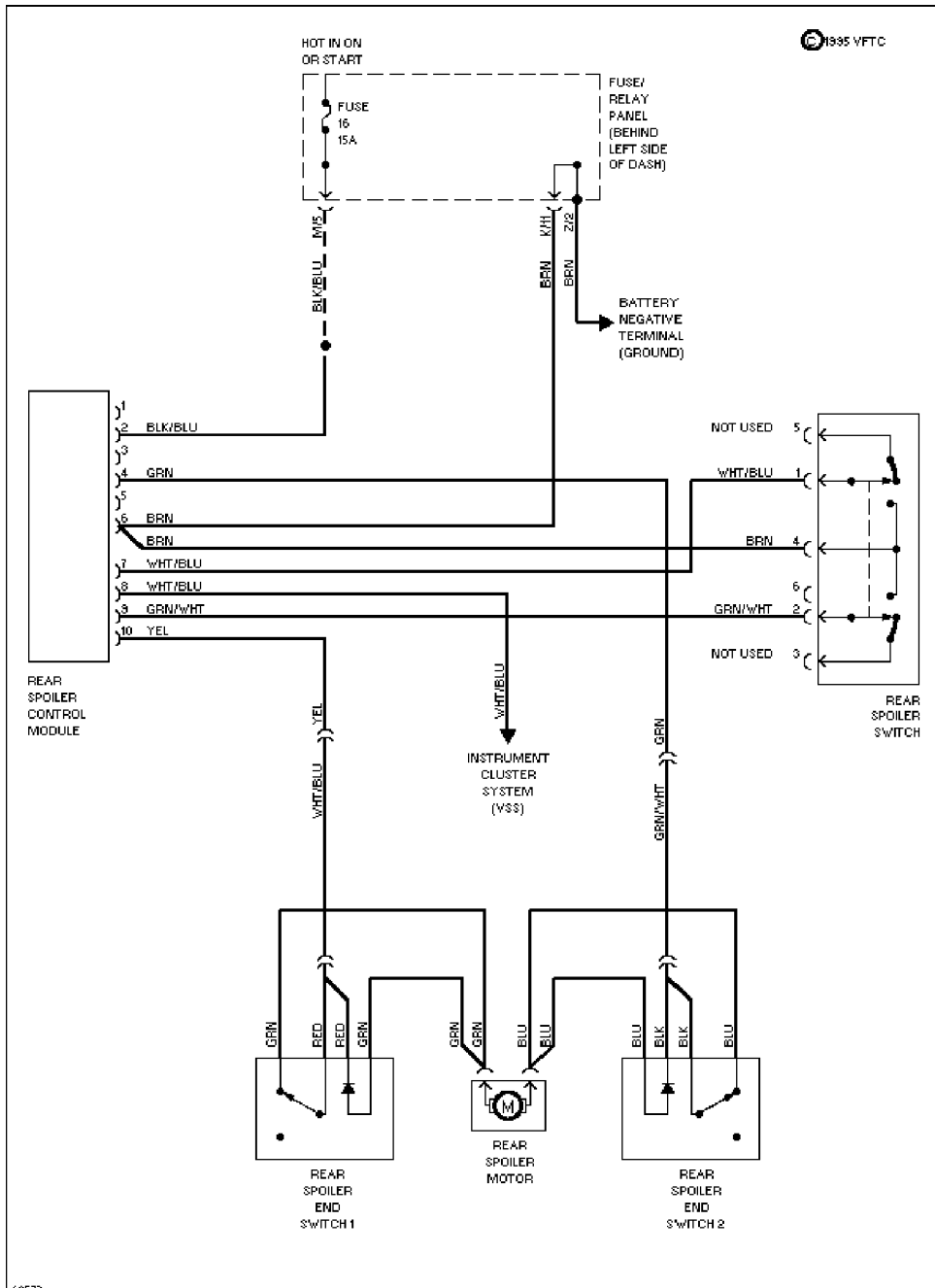
Active Aerodynamic Circuit
