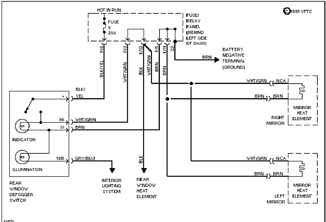
Heated Mirrors Circuit
