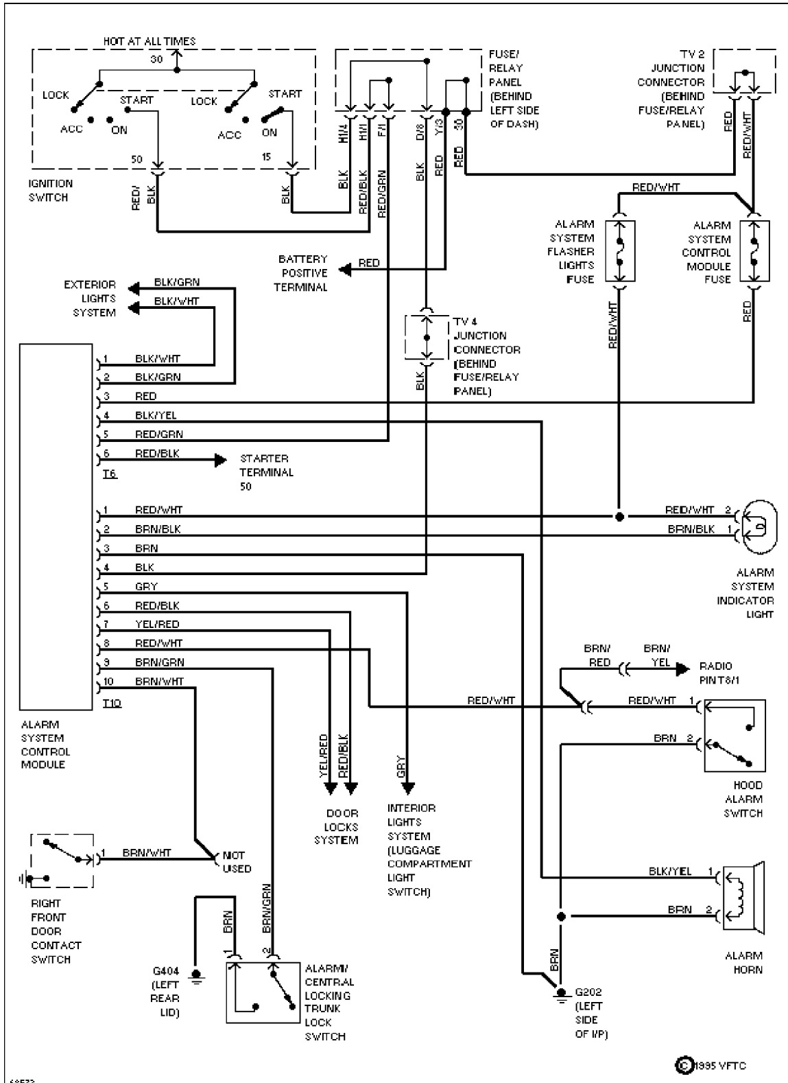
Anti-theft Circuit
