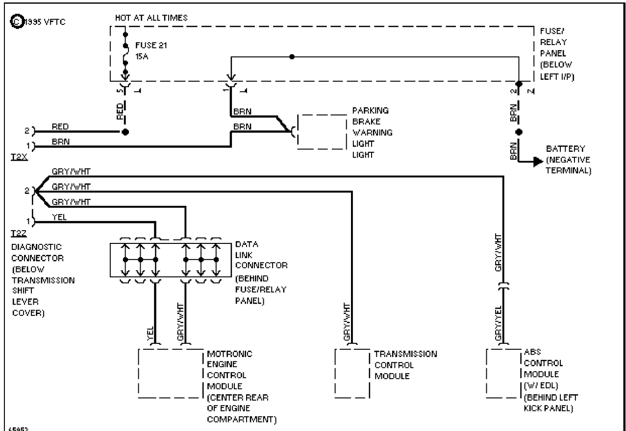
Computer Data Lines
