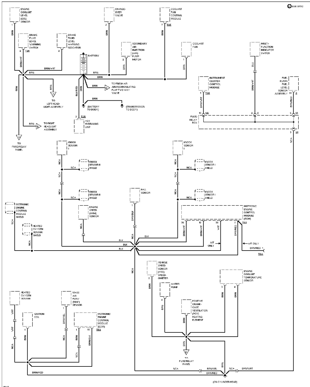
Ground Distribution Circuit (1 of 5)
